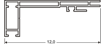
26.55 LIGHT BOX 120 (T8) BLACK
