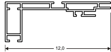
26.55 LIGHT BOX 120 (T8)
