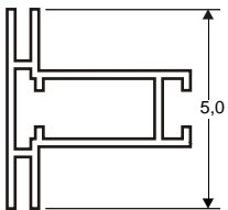
20.15 DOUBLE SIDED FRAME 50
