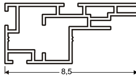
26.40 LIGHT BOX 100 (T8)
