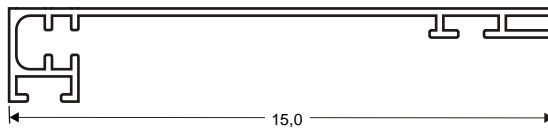
26.59 LIGHT BOX 150 Heavy Duty (T8)
