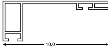
26.57 LIGHT BOX 150 (T8)
