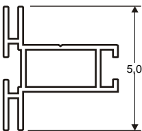
20.72 DOUBLE SIDED FRAME 50
